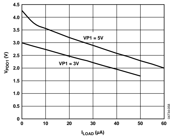
Figure 12. V PDO1 (Weak Pull-Up to VPn) vs. I LOAD
