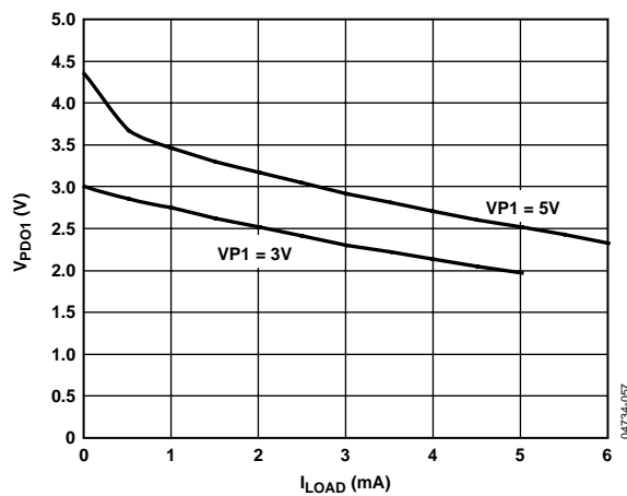
Figure 11. V PDO1 (Strong Pull-Up to VPn) vs. I LOAD
